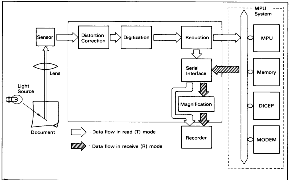
Figure 1 DIPP Function
